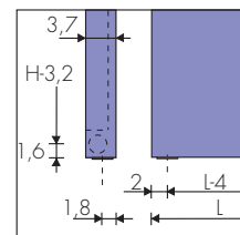
SO-FLEX-FXH 180/220.. ▲▽ t. c.= L-4 cm
