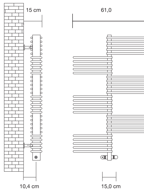
Inter-axis between connectors with sizes based on Tubes valves
