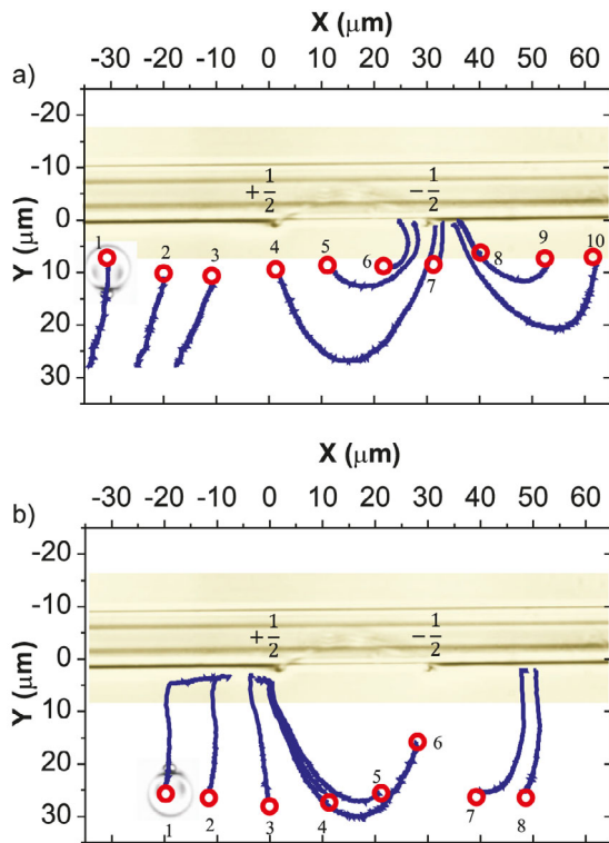
Fig. 20. Trajectories of dipolar colloids in the vicinity of a charge-neutral loop, after it was released from the optical trap towards the fiber. (a) The + end of the dipole is near the fiber. The lines 1-3 show the repulsive trajectories due to the topological soliton close to the charge-neutral loop. The lines 4 and 5 show the dipole trajectories when the particle is repelled by the + end of the loop and topological soliton, and attracted to the - end of the loop. The lines 6-8 show the attractive trajectories towards the - end of the loop. The lines 9 and 10 indicate the trajectories of the dipole with repulsive interaction caused by the topological soliton and attractive interaction caused by the - end of the loop. (b) The - end of the dipole is near the fiber. The lines 1-4 show the attractive trajectories towards the topological soliton and + end of the loop. The lines 5 and 6 present the repulsive interaction due to the - end of the loop and attractive interaction due to the + end of the loop and topological soliton. The lines 7 and 8 indicate the attractive trajectories towards the topological soliton. Open circles indicate the starting positions.
