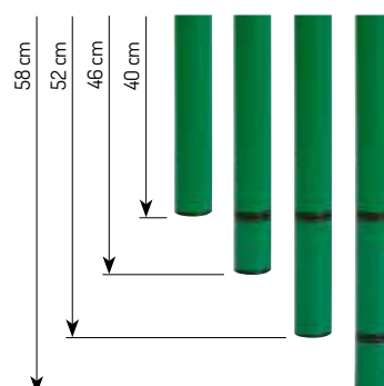
Height adjustment
