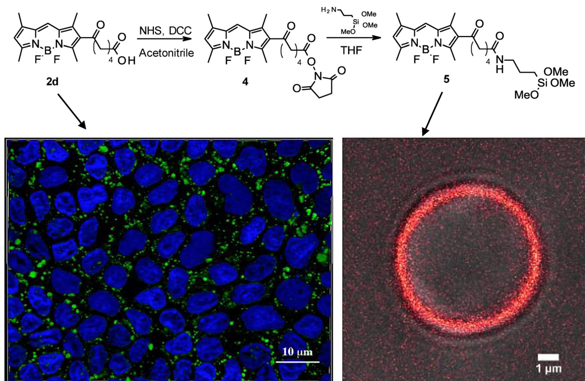
Figure 3. Reaction scheme for the preparation of a trimethoxysilane bearing BODIPY 5 . a) MDCK confluent cell culture treated with 2d (green). The nuclei were stained with DAPI (blue) and live cells were labelled with 0.5 mM 2d (stock solution 5 mM in DMSO and then diluted 1:10 in ADMEM medium); the cells were then fixed in 4% formaldehyde. b) Superimposition of fluorescence and bright-field images of a 7.3 \mu\text{m} silica colloid treated with 5 and dispersed in a low birefringent liquid crystal mixture CCN47-55. Fluorescence was imaged with excitation at 470 nm and emission was detected in the range of 495–574 nm (in this case the red color merely indicates high emission and does not reflect the real color of the light emitted).
