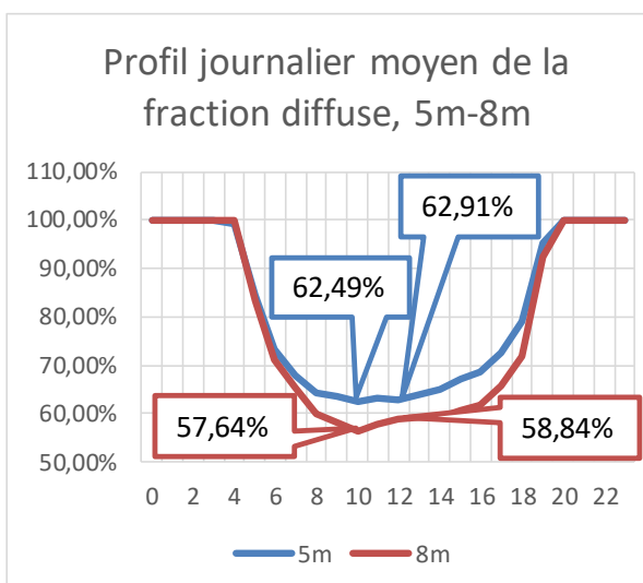
Figure 21 : Fraction diffuse horaire, 5m-8m
