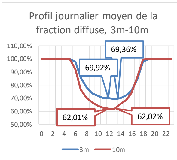
Figure 19 : Fraction diffuse horaire, 3m-10m
